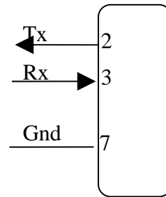
PC 25 Way D-Type Male
