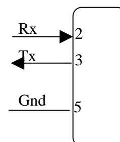
PC 9 Way D-Type Male
