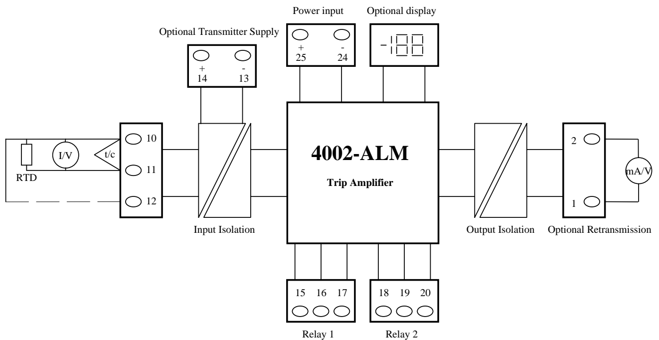
FIG. 1 - BLOCK SCHEMATIC DIAGRAM FOR THE IIR-4002-ALM TRIP AMPLIFIER
